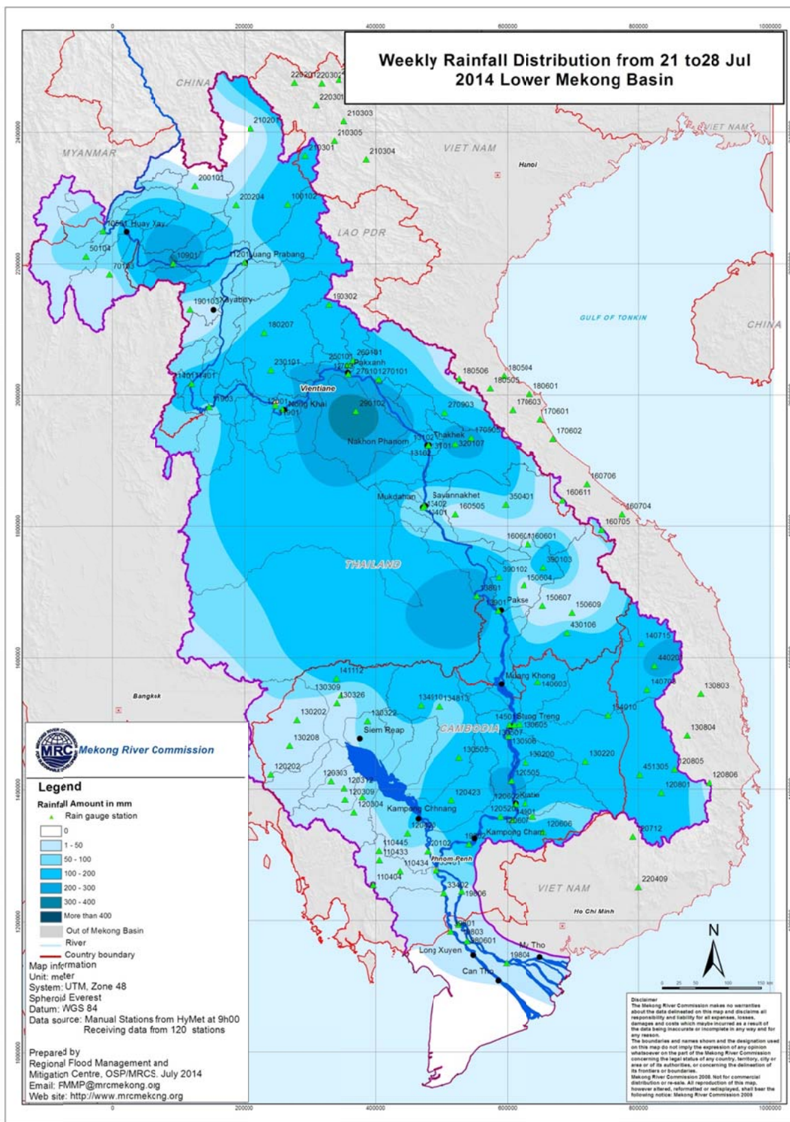
Figure 3: Weekly Rainfall Distribution from 21 st – 28 th July 2014 over the LMB
