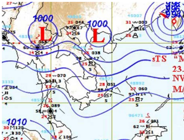
Figure 1: Weather map for 22 nd July 2014
