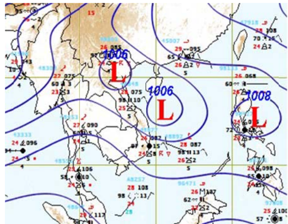
Figure 2: Weather map for 26 th July 2014
